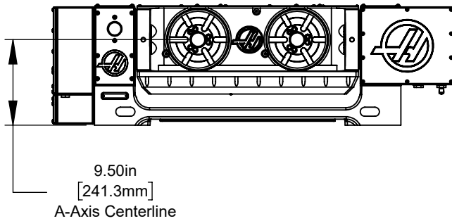
Front View Platter Rotated 90° to Base
